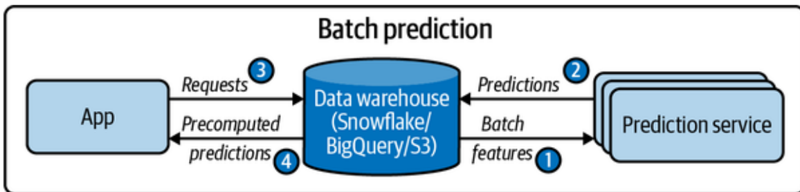
Figure 7-4. A simplified architecture for batch prediction
