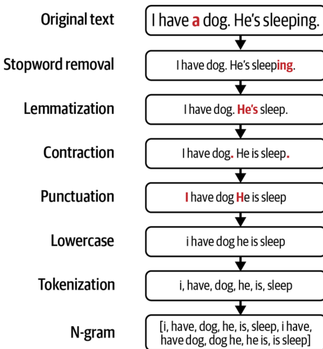
Figure 5-1. An example of techniques that you can use to handcraft n -gram features for your text
