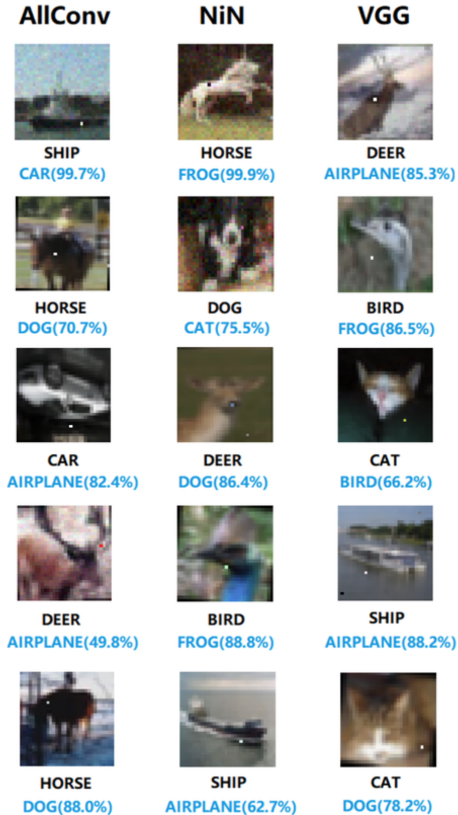
Figure 4-12. Changing one pixel can cause a neural network to make wrong predictions. The three models used are AllConv, NiN, and VGG. The original labels made by those models are above the labels made after one pixel was changed. Source: Su et al. 50
