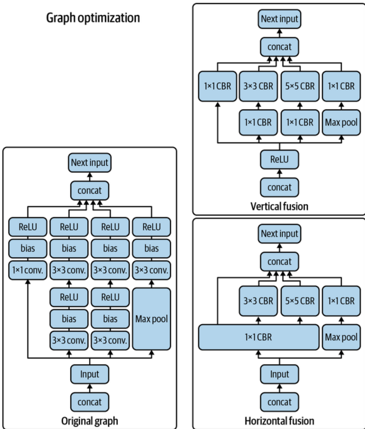
Figure 7-14. Vertical and horizontal fusion of the computation graph of a convolution neural network. Source: Adapted from an image by TensorRT team 48
